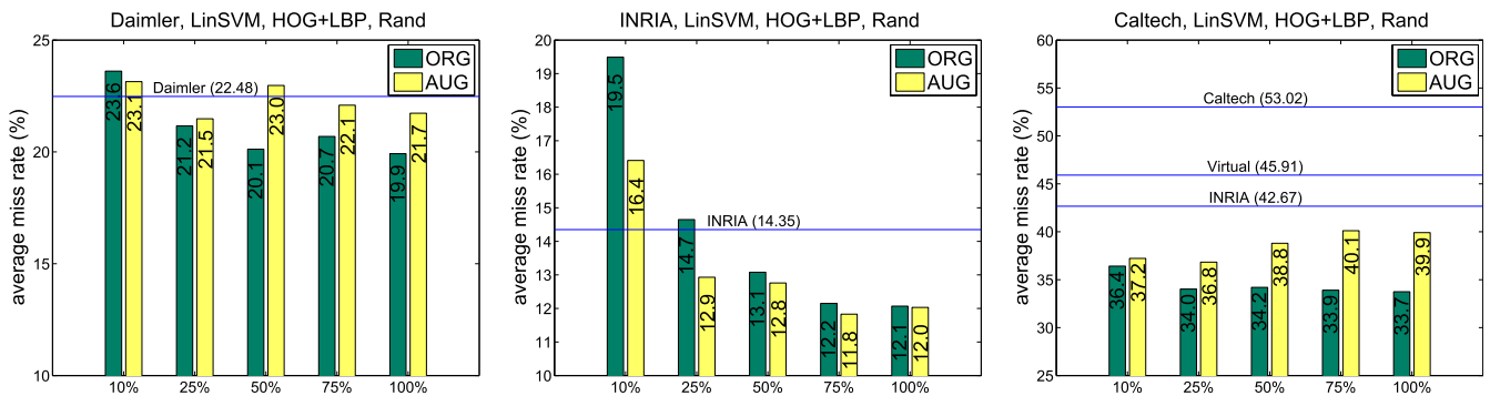
Fig. 6. AMRs of progressively adding more (10-100 percent) target domain (real-world) training pedestrians to the virtual-world ones. Lines mark the AMR for detectors trained with the 100 percent of the indicated training set.
